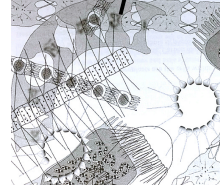
Phytoplankton – Microscopic plants
